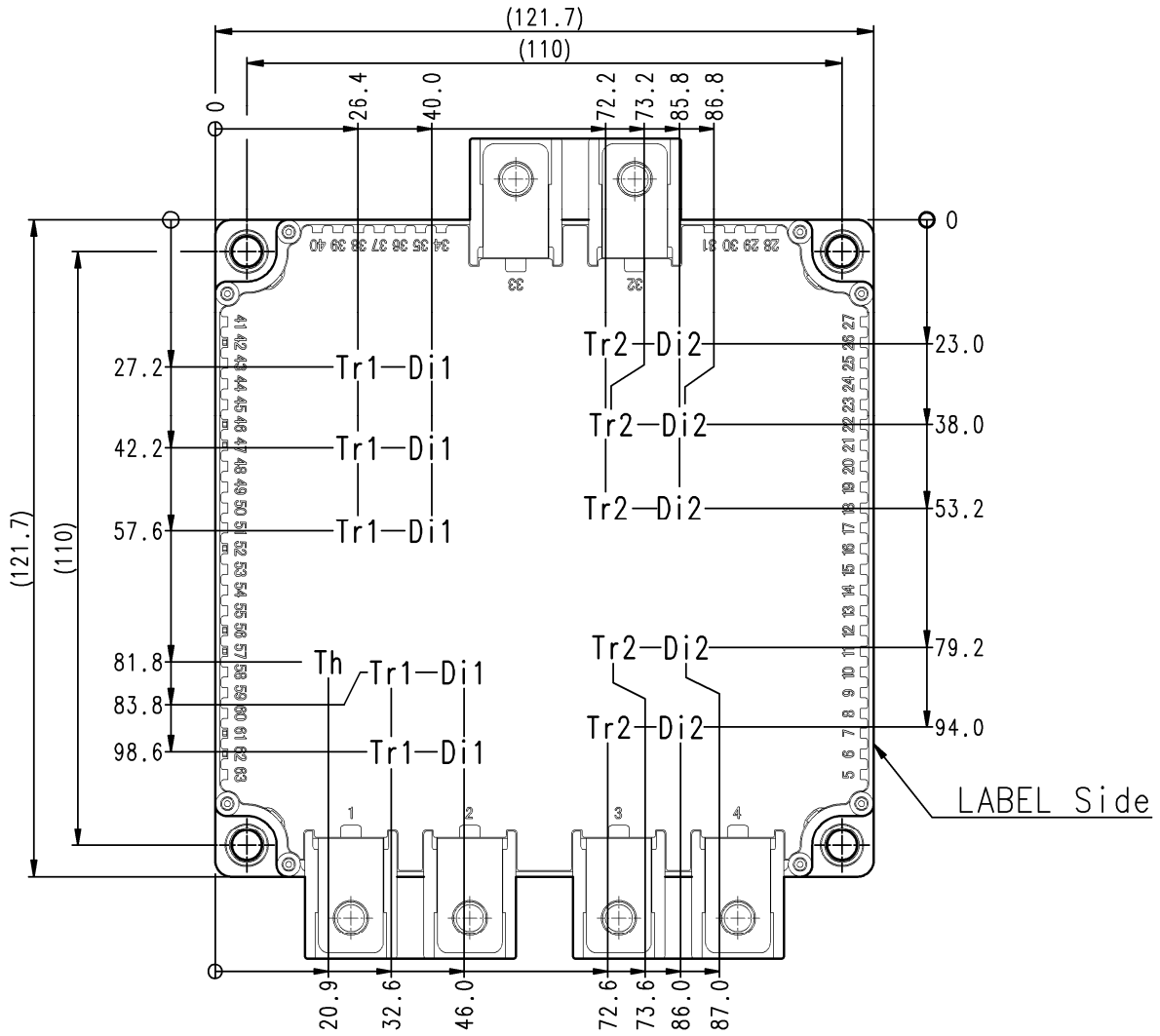
Tr1/Tr2: IGBT, Di1/Di2: FWDi, Th: NTC thermistor
