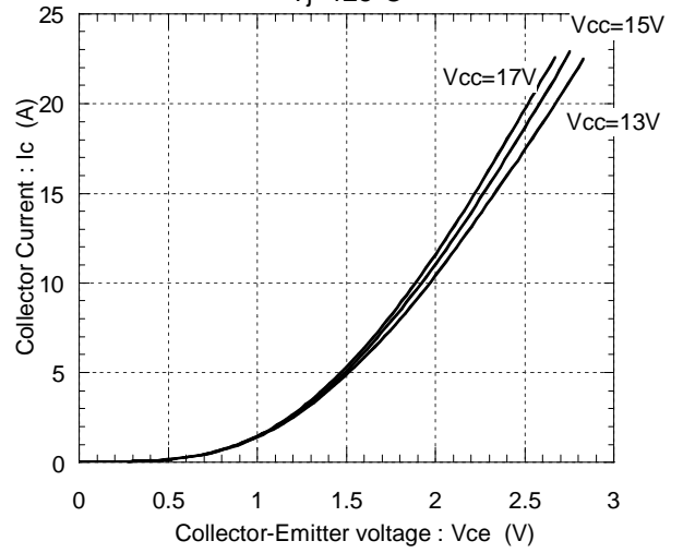
Collector current vs. Collector-Emmitter voltage Tj=125°C
