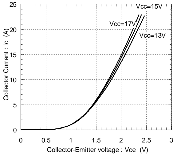
Collector current vs. Collector-Emmitter voltage Tj=25°C
