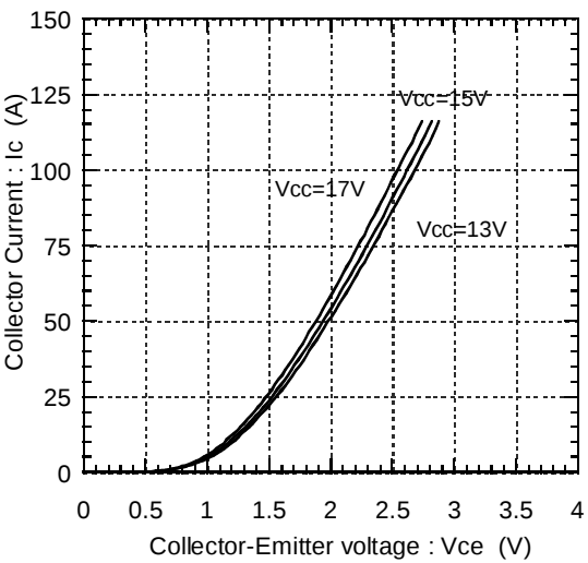
Collector current vs. Collector-Emitter voltage (typ.) Tj=25°C(Terminal)
