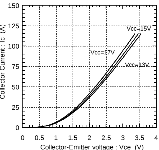
Collector current vs. Collector-Emitter voltage (typ.) Tj=125°C(Terminal)
