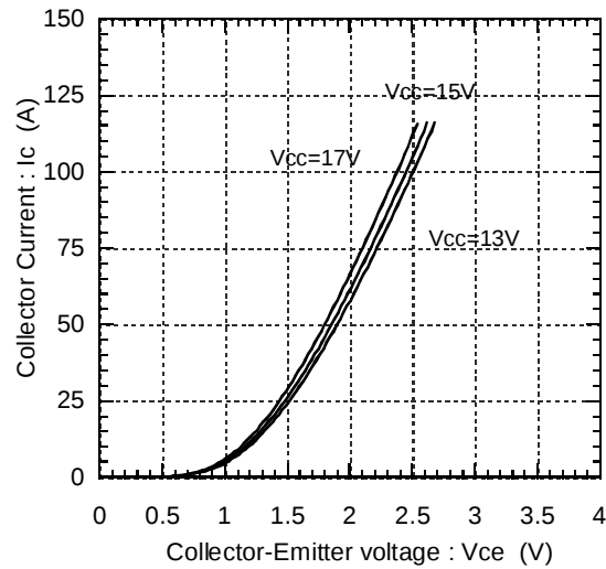
Collector current vs. Collector-Emitter voltage (typ.) Tj=25°C(Chip)
