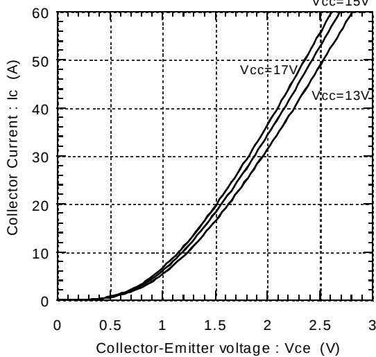
Collector current vs. Collector-Emitter voltage T_j=125^{\circ}\text{C} (Chip)
