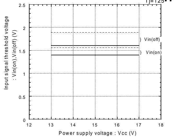
Input signal threshold voltage vs. Power supply voltage
