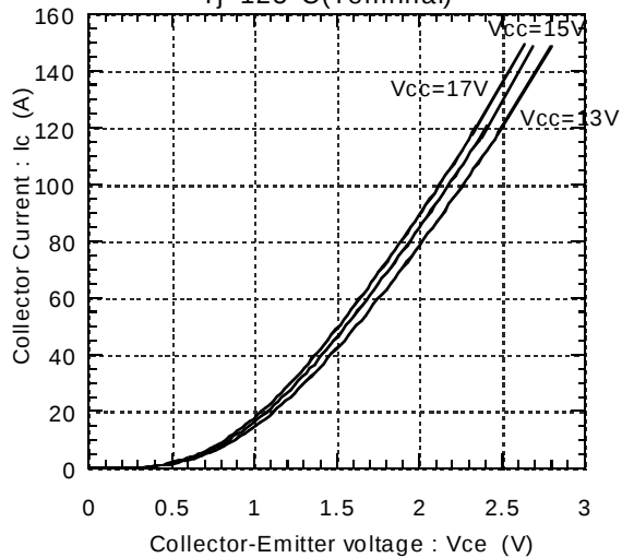
Collector current vs. Collector-Emitter voltage T_j=125^{\circ}\text{C}(\text{Terminal})
