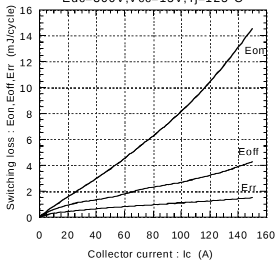
Switching Loss vs. Collector Current Edc=300V,Vcc=15V,Tj=125°C
