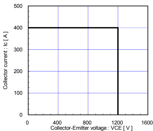
Reverse bias safe operating area (max.) +V_{GE}=15V, -V_{GE} \le 15V, R_G \ge 3.0\Omega, T_j \le 125^\circ C
