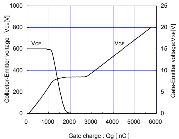
Dynamic Gate charge (typ.) VCC=600V, Ic=1200A, Tj= 25°C
