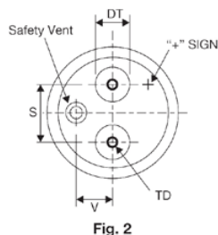
Terminal styles A (ø36mm only), C, G, J, M
